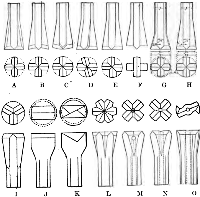
Fig. 4. Types of Machine Drill Bits.
